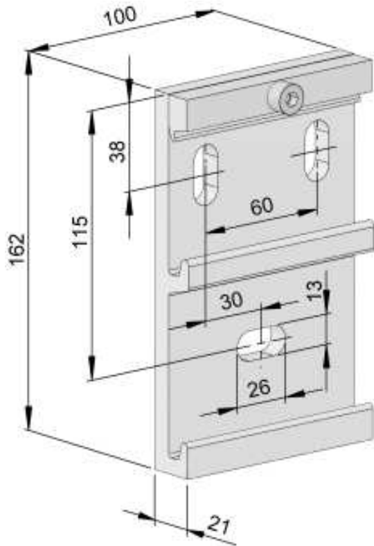
Wall Bracket
