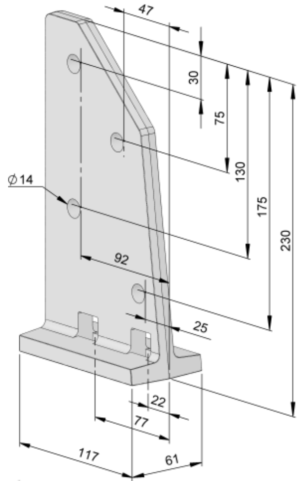
Joist Attachment
