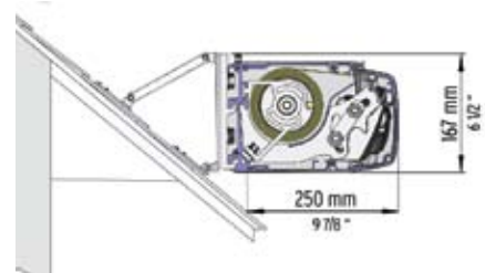
Roof Mount
