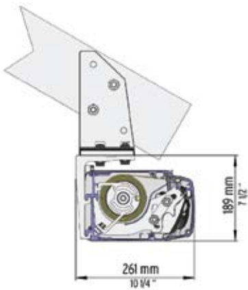
Joist Mount
