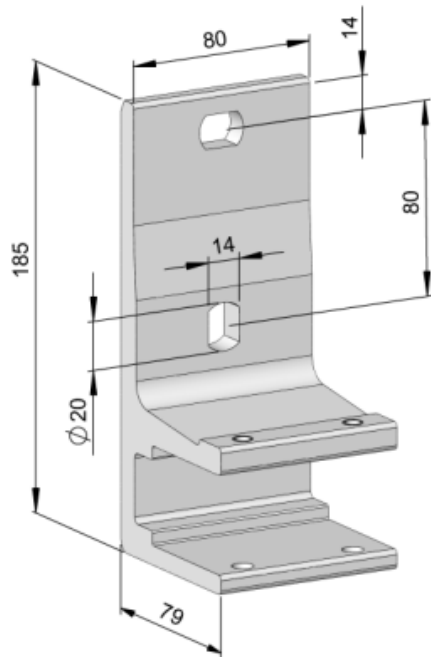
Soffit Bracket
