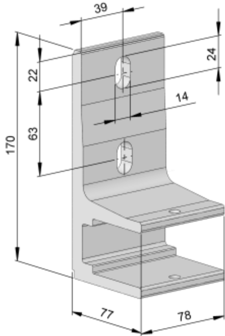
Wall Bracket
