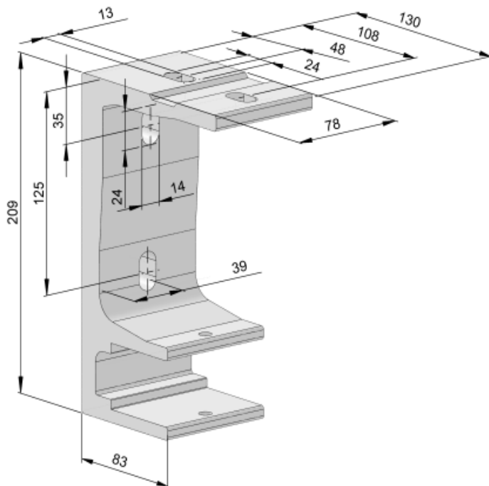
Soffit Bracket
