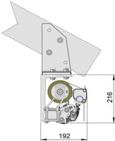
Joist Mount
