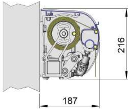
Wall Mount
